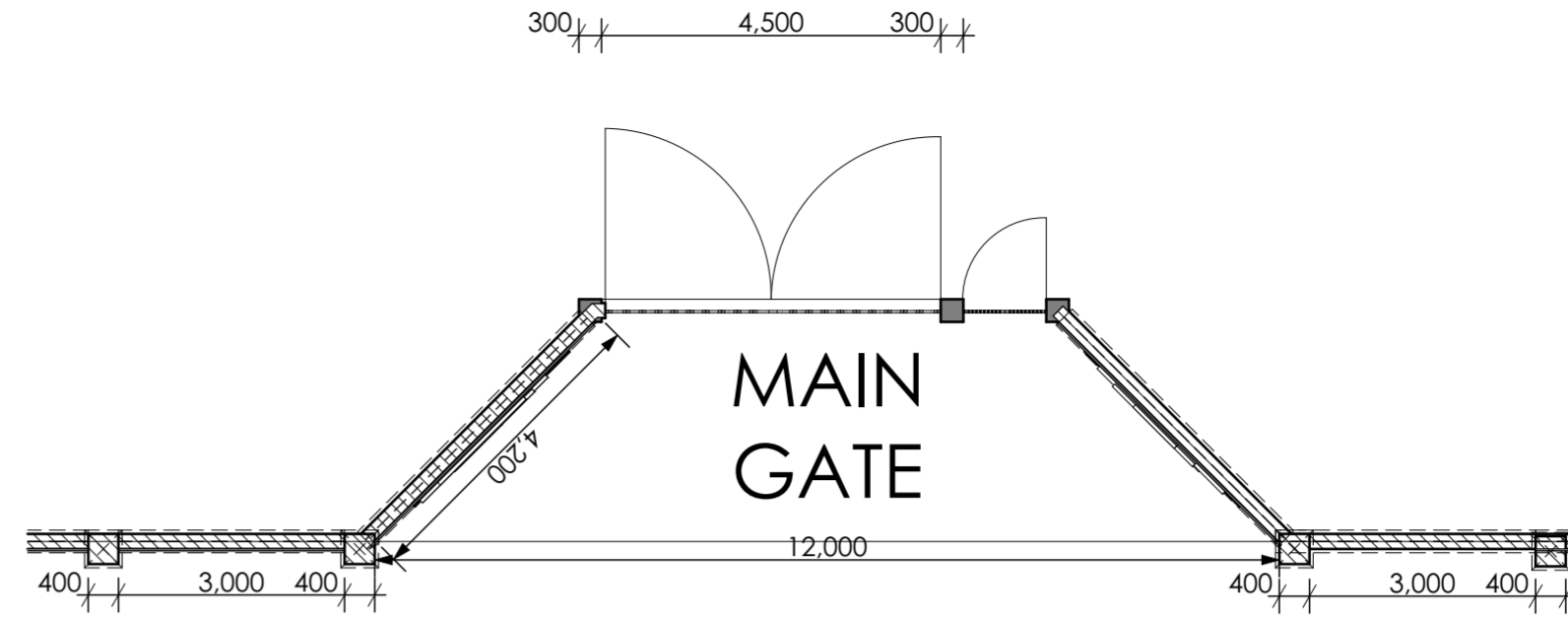
GATE FLOOR PLAN
